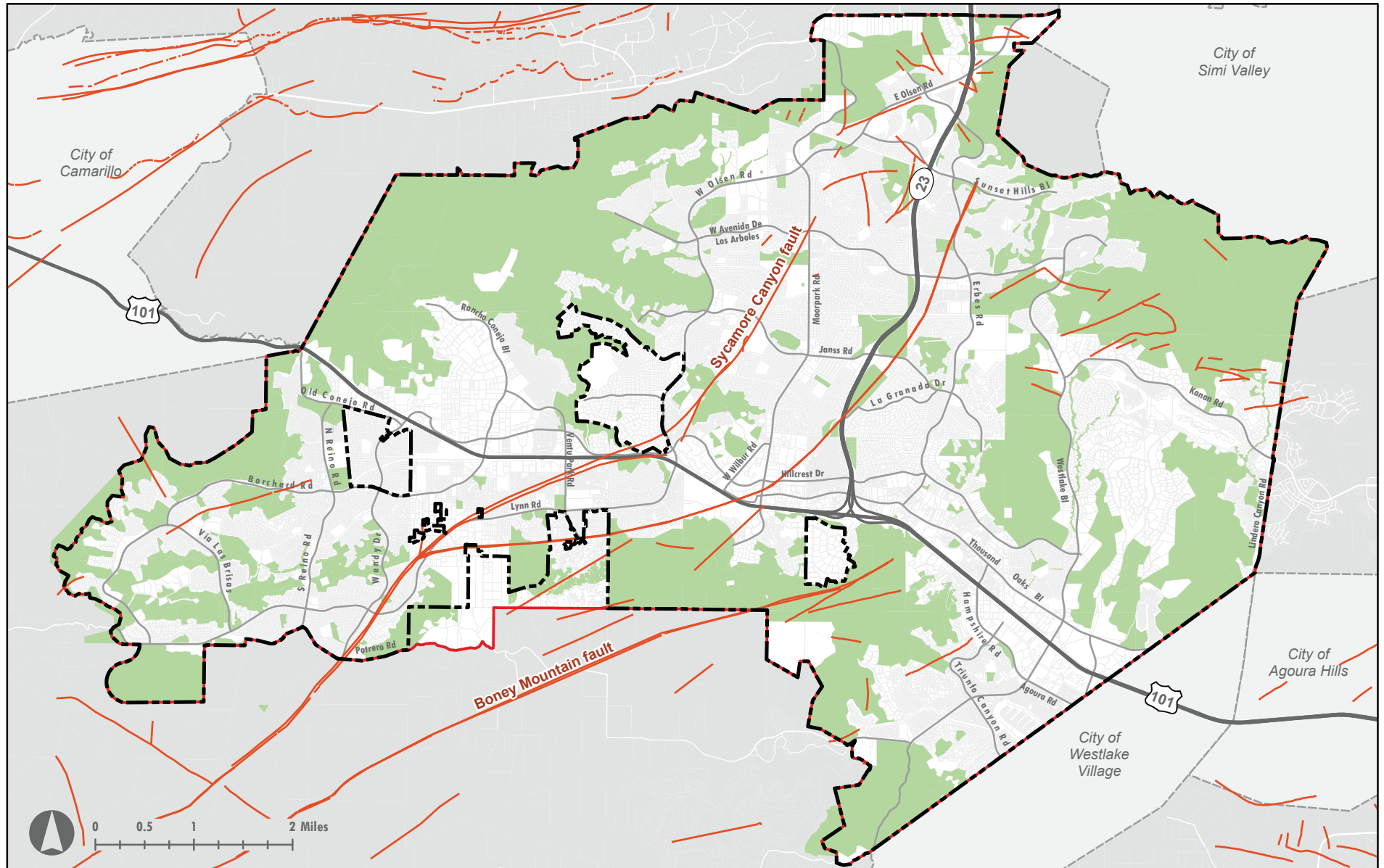
FIGURE 10.1 Seismic Faults
